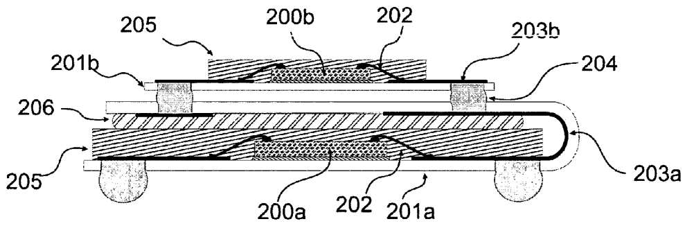
Prior Art
